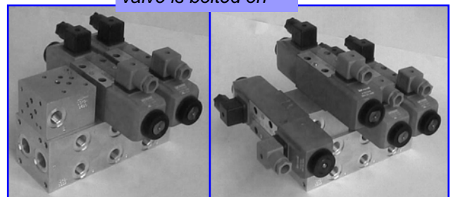
Add-on Sandwich assembly before and after the add-on valve is bolted on
